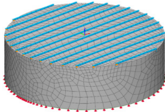
FEA MODEL OF SHELL + ROOF AND SUPPORT BEAMS
