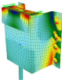
TANK ANCHORAGE FEA VALIDATION
